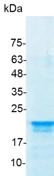
SDS-PAGE analysis of recombinant human FGF-18
