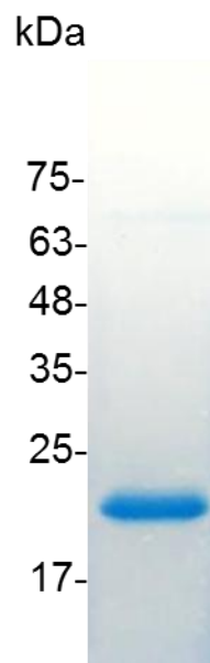
SDS-PAGE analysis of recombinant human FGF-2
