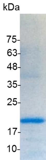
SDS-PAGE analysis of recombinant human IFN omega
