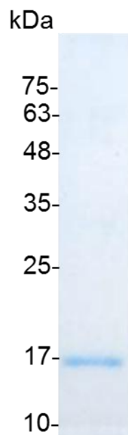
SDS-PAGE analysis of recombinant human IFN gamma
