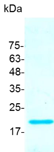
SDS-PAGE analysis of recombinant human TNF beta
