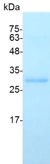
SDS-PAGE analysis of recombinant mouse HMGB1
